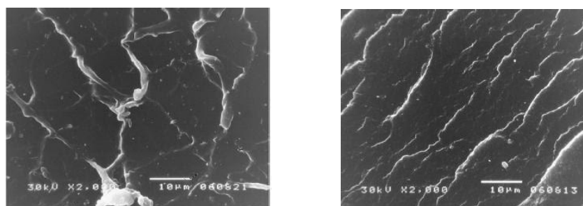
Figure 1: SEM micrographs of NBR rubber vulcanisates
